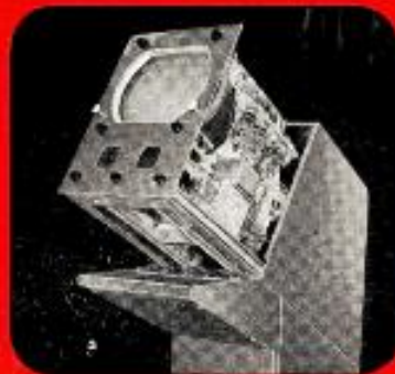
✓ Counter-balanced "draw-out" and removable panels for accessibility. ✓ 12 1/2" aluminized picture tube.
